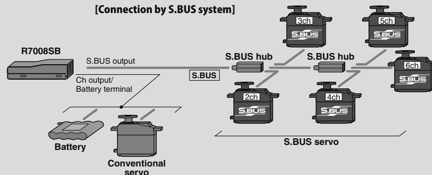
[Connection by S.BUS system]
